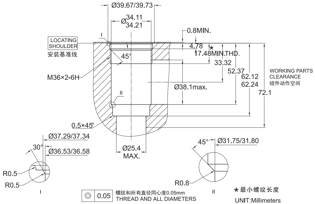
CAVITY: SUN T-16A
