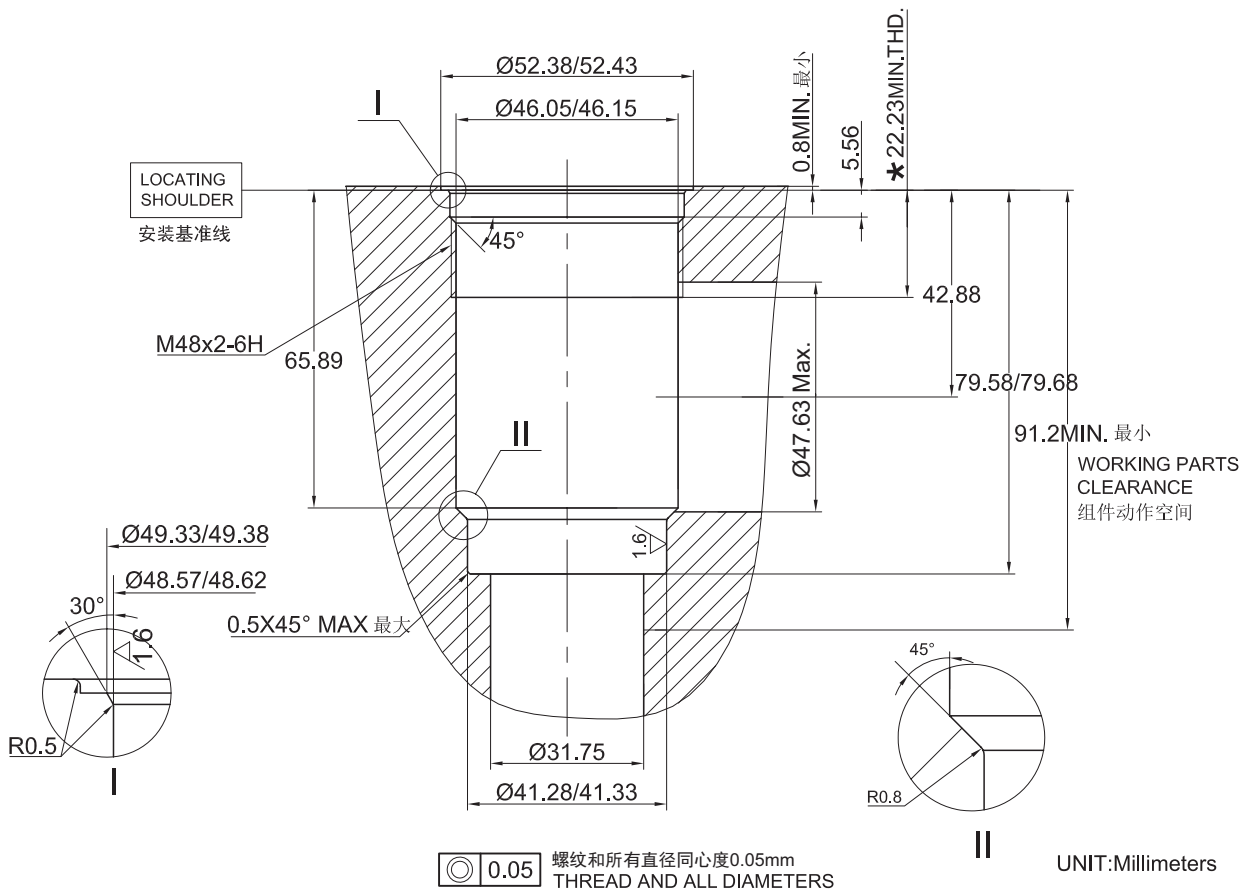
CAVITY: SUN T-18A
